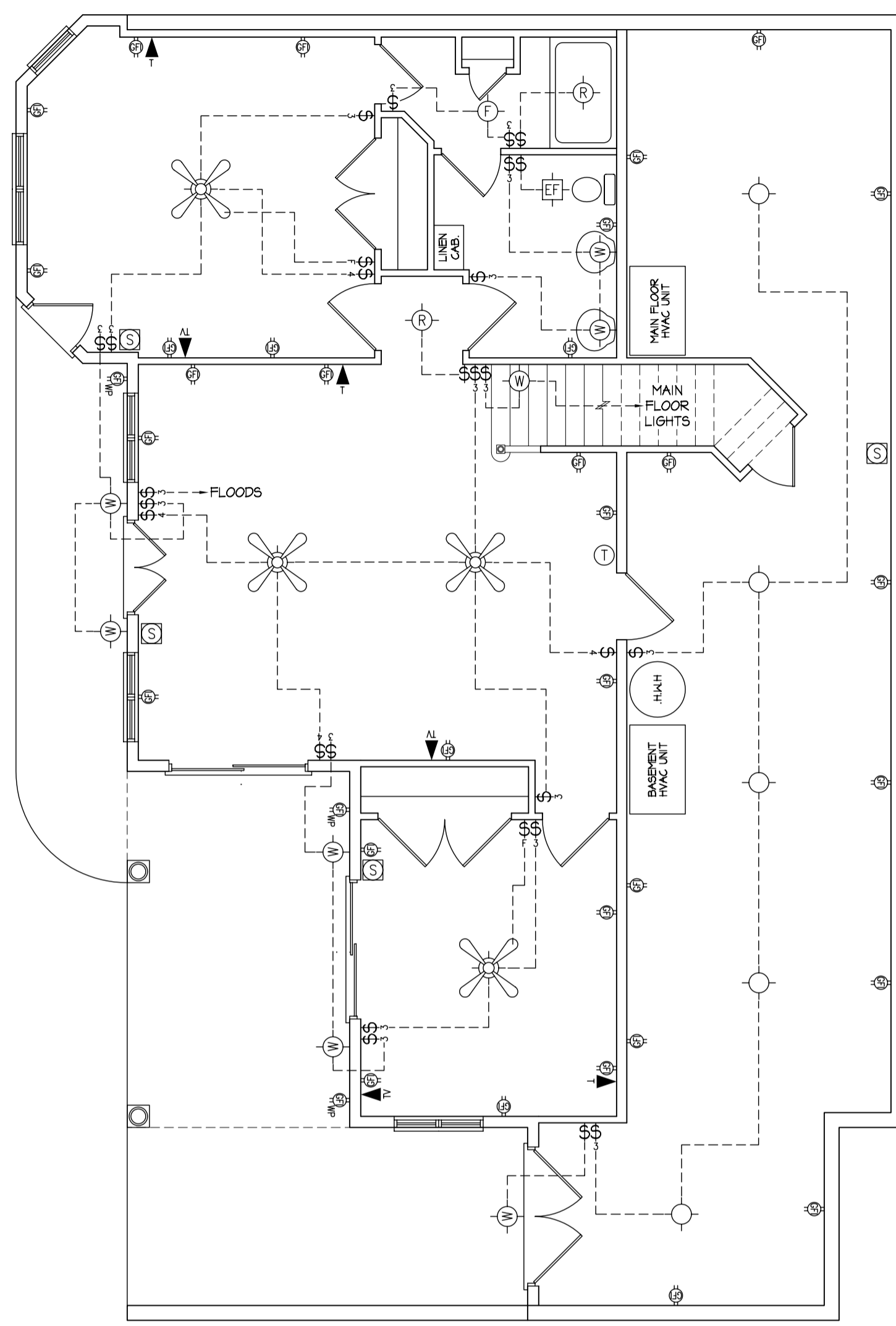
BASEMENT ELECTRICAL SCALE: 3/16" = 1'-0"
