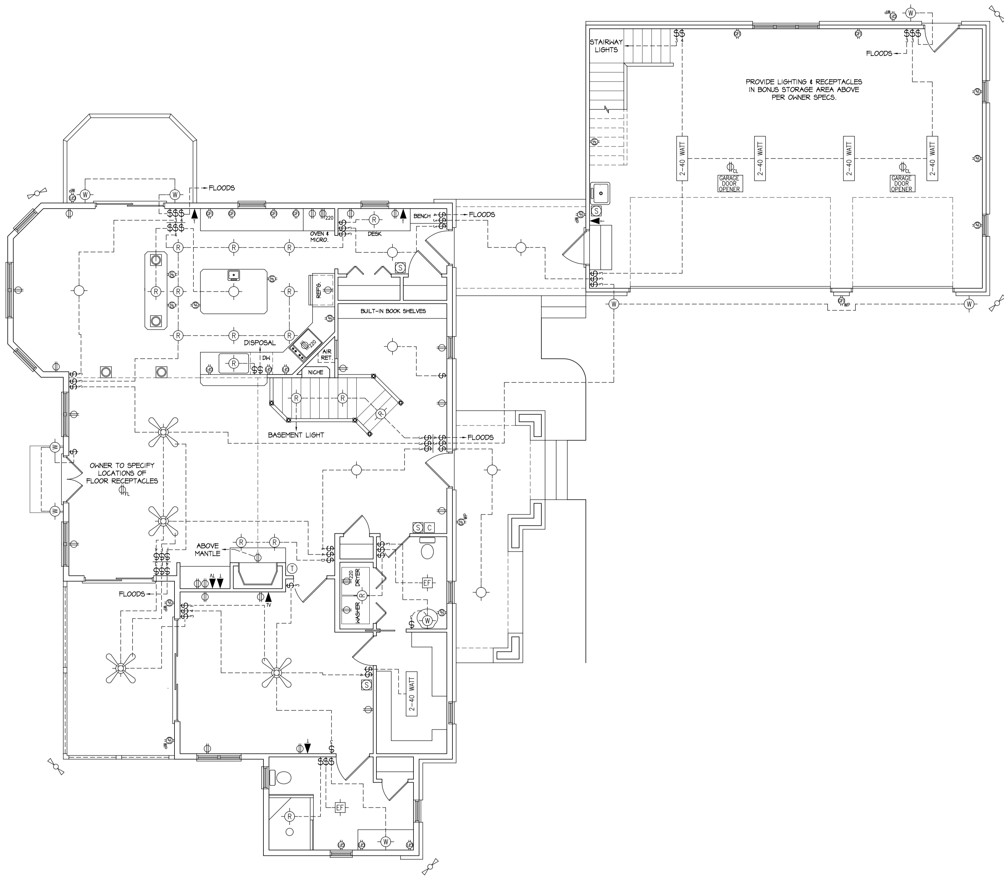
MAIN FLOOR ELECTRICAL SCALE: 3/16" = 1'-0"
